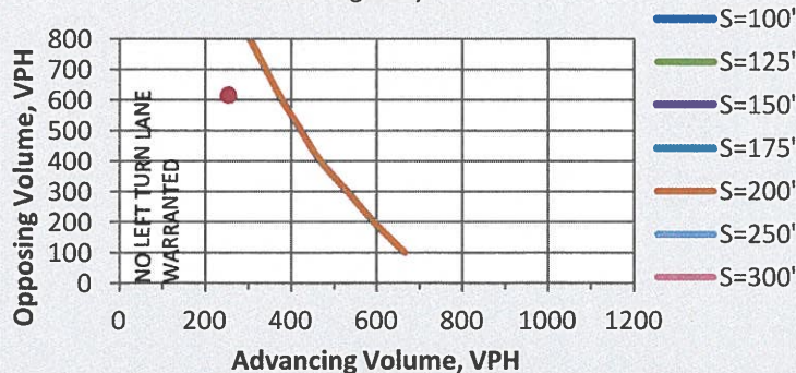
Warrant for Left-Turn Storage Lane 2-Lane Highway
