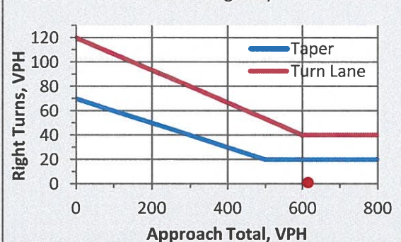
Warrants for Right Turn Treatments 2-Lane Highway
